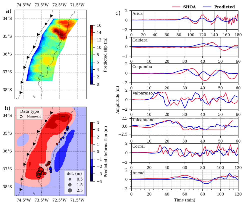
Figure 3.4.1: Figure a) Final estimation of heterogeneous slip distribution model for 2010 earthquake. Figure b) Vertical deformation field for 2010 earthquake. Deformation data numerical (circle) observations are also shown. Red markers indicate uplift, blue markers indicate subsidence. Figure c) Wave amplitude from predicted (blue lines) and SHOA (red lines) tide gauges.
