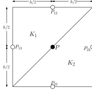
Figure 4.3: Positions of the degrees of freedom in the stencil of the first type.
