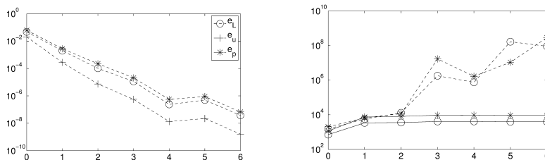
Figure 2.6: Left: Errors e_L ( \circ ), e_u ( + ) and e_p ( * ) versus k = 0, \dots, 6 in semi-log scale, for 154 elements. Right: Ratios r^{\kappa} (dashed line) and r^{\kappa}_{poly} (solid line) in semi-log scale for 28 ( \circ ) and 154 ( * ) elements.
