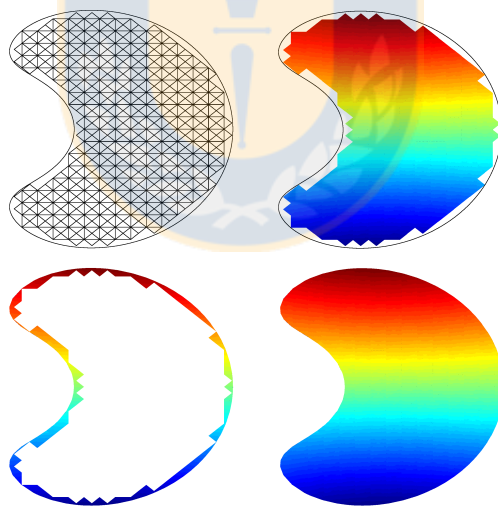
Figure 2.5: Approximation of the first component of L in Example 3 for k = 2 and 712 elements.
