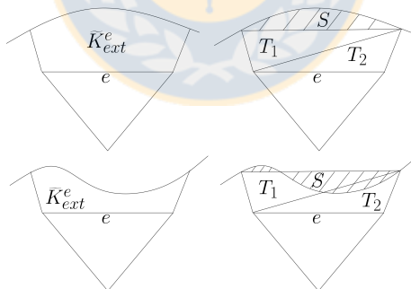
Figure B.1: Examples of \tilde{K}_{ext}^e divided in triangles T_1 and T_2 , and a region S (dashed area).
