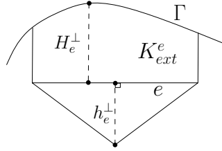
Figure 1.1: Example of a region K_{ext}^e and the distances H_e^\perp and h_e^\perp .
