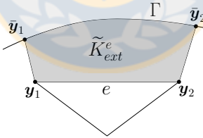
Figure 2.1: Example of points \bar{\mathbf{y}}_j associated to the vertices \mathbf{y}_j and region \tilde{K}_{ext}^e .
