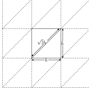
Figure 4.1: Sketch of the mesh.
