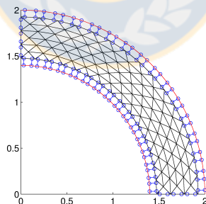
Figure 2.3: Domain \Omega (red solid line) and D_h in Example 2. Transferring paths (blue solid lines) associated to the quadrature points when k = 1 .
