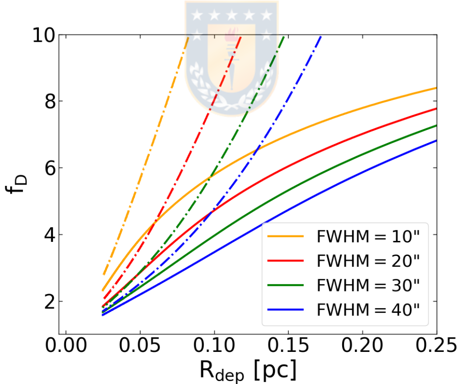
Figure 3.9: f_D variation as a function of R_{\text{dep}} for the best-fitting model applied to clump-5. Full lines represent the f_D - R_{\text{dep}} relation assuming f_D = 10 for R < R_{\text{dep}} , while the dash-dotted line are the ones for f_D = \infty . The blue profile in Fig. 3.8 (a) was convolved at different angular resolutions in order to predict how the same relation changes with different observational conditions. Colours are linked to the different FWHMs used for the convolution.
