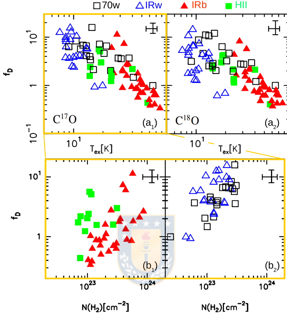
Figure 2.6: Panels (a) show CO depletion factors from ^{12}\text{C}^{17}\text{O} (on the left) and ^{12}\text{C}^{18}\text{O} (on the right) as a function of T_{ex} for the TOP100 sample. Panels (b) show the CO depletion factor (from ^{12}\text{C}^{17}\text{O} ) as a function of N(\text{H}_2) , for the TOP100 sample. A typical uncertainty is shown in the top right corner of each panel. Each evolutionary class is shown with a different symbol and colour, as indicated. This Figure is adapted from Figures 8 and 9 of Giannetti et al. (2014).
