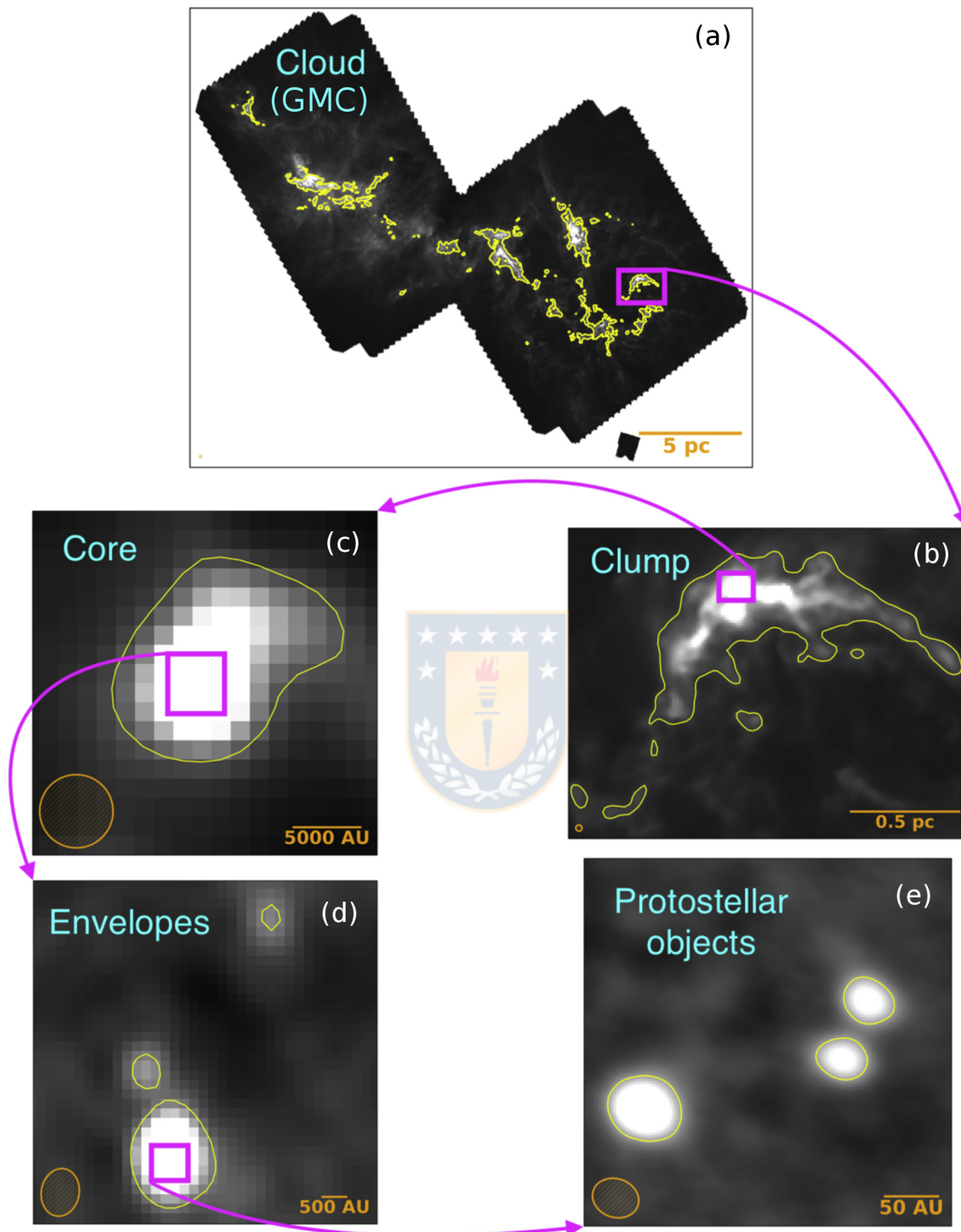
Figure 1.2: Hierarchical cloud structures in the Perseus molecular cloud. Panel (a) shows the whole GMC scale observed with Herschel at 350\ \mu\text{m} , where seven clumps were detected (see also Sadavoy et al. 2014; Mercimek et al. 2017). Panel (b) is a zoom of one of those clumps (L1448; Kwon et al. 2006). Panel (c) reports the SCUBA 850\ \mu\text{m} map of one of the cores that resides in L1448 (J032536.1+304514; see Di Francesco et al. 2008). Panel (d) reveals the three envelope-fragments observed with the Submillimetre Array (SMA) in J032536.1+304514, one of those harbouring three protostellar objects (Panel e observed with the Very Large Array; Tobin et al. 2016). This figure is adapted from Fig. 2 of Pokhrel et al. (2018).
