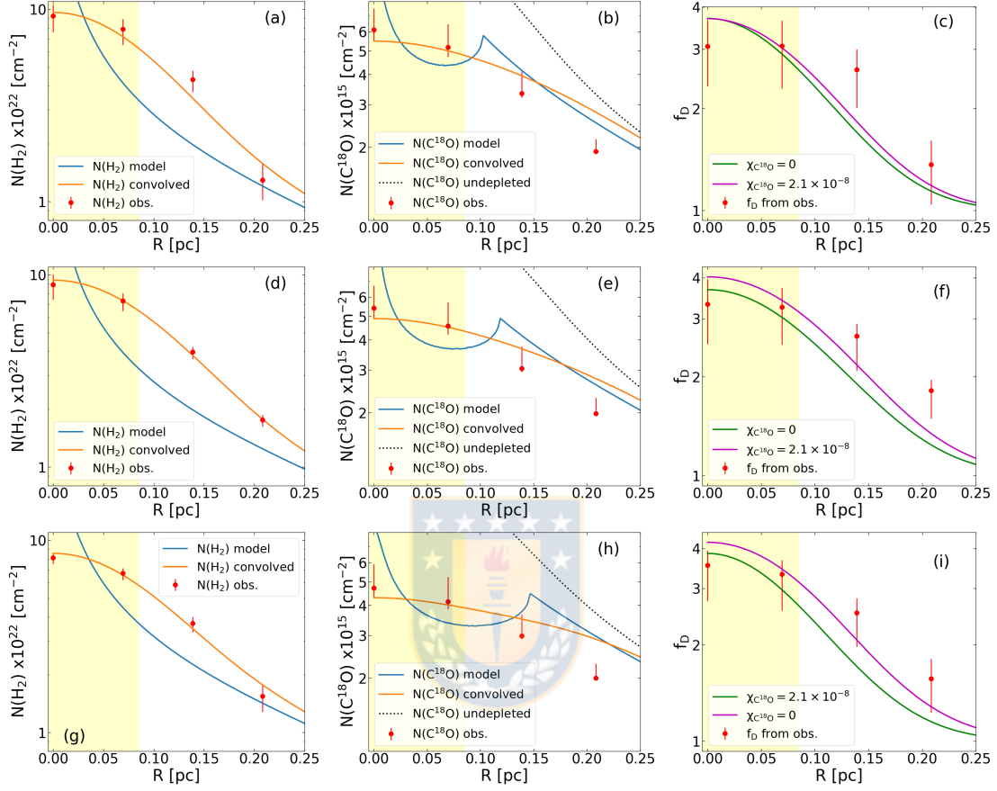
Figure 3.8: From top: Column density profiles of \text{H}_2 and \text{C}^{18}\text{O} in panel (a) and (b), respectively, while panel (c) shows the los- and beam-averaged depletion factor profile from region C5 in Fig. 3.1. Panels (d), (e) and (f) are the same as (a), (b) and (c), respectively, for region C7, while panels (g), (h) and (i) refer to the region F1. Blue profiles in panels (a), (d) and (g) are the synthetic column densities profiles obtained by the integration of the number densities distribution; solid-blue lines in panels (b), (e) and (h) are the same for \text{C}^{18}\text{O} assuming \chi_{\text{C}^{18}\text{O}} = 2.1 \times 10^{-8} for R < R_{\text{dep}} , and the estimated position of R_{\text{dep}} corresponds to the cusp. Orange profiles in panel (a), (b), (d), (e), (g) and (h) are the convolution results of the blue profiles and the Herschel beam at 500\mu\text{m} , while black-dotted line in panel (b), (e) and (h) indicates the convolved undepleted-profile of N(\text{C}^{18}\text{O}) assuming a constant \chi_{\text{C}^{18}\text{O}} = 2.1 \times 10^{-7} . Green and magenta profiles in panel (c), (f) and (i) show the depletion factor profiles obtained by assuming different abundances for R < R_{\text{dep}} (see Eq. 3.5). Red points are the observed values for each quantity plotted. The yellow-shaded area shows the dimensions of the Herschel HWHM at \lambda = 500 \mu\text{m} (i.e. FWHM= 36'' ; 0.17 pc at the source distance). All profiles are plotted as a function of the radial distance from the spine.
