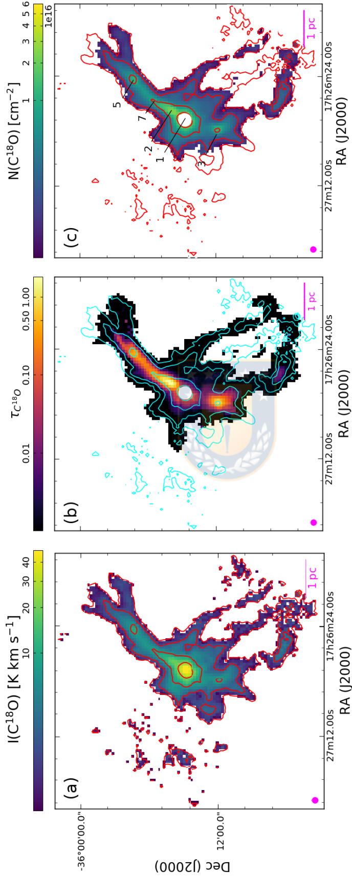
Figure 3.3: (a) Integrated intensity distribution of the C^{18}O J = 2 - 1 molecular line transition detected with APEX in units of K km s^{-1} . (b) Map of the opacity from the N(H_2) map, following the procedure described in Sect. 3.2.2. The final \tau-N(H_2) relation used is: \log_{10}(\tau_{C^{18}O}) = 2.5 \log_{10}(N(H_2)) - 57.4 . (c) C^{18}O column density map obtained from the integrated intensity distribution, shown in Fig. 3.3 (a), using Eq. (3.1). The red and cyan contours are the 3, 9, 27 and 81 \sigma contours of the integrated flux density distribution in panel (a), where 3\sigma = 0.9 K km s^{-1} .
