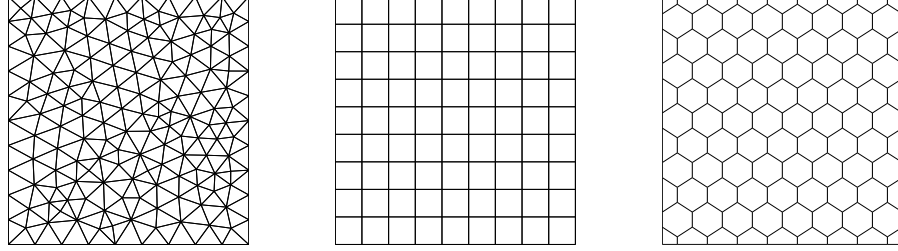
Figure 4.1: Sample meshes: \mathcal{T}_h^1 (left), \mathcal{T}_h^2 (middle) and \mathcal{T}_h^3 (right). In all of them N = 9 .
