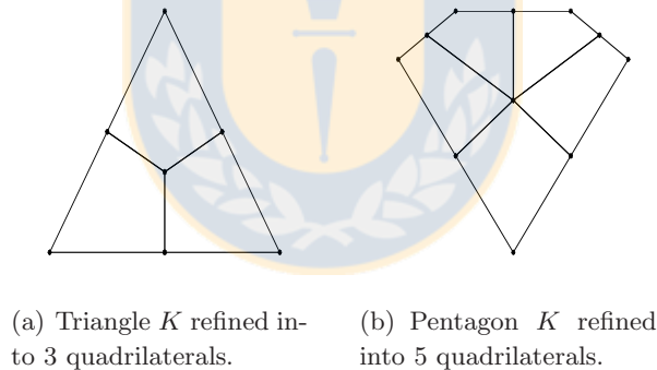
Figure 3.1: Example of refined elements for VEM strategy.
