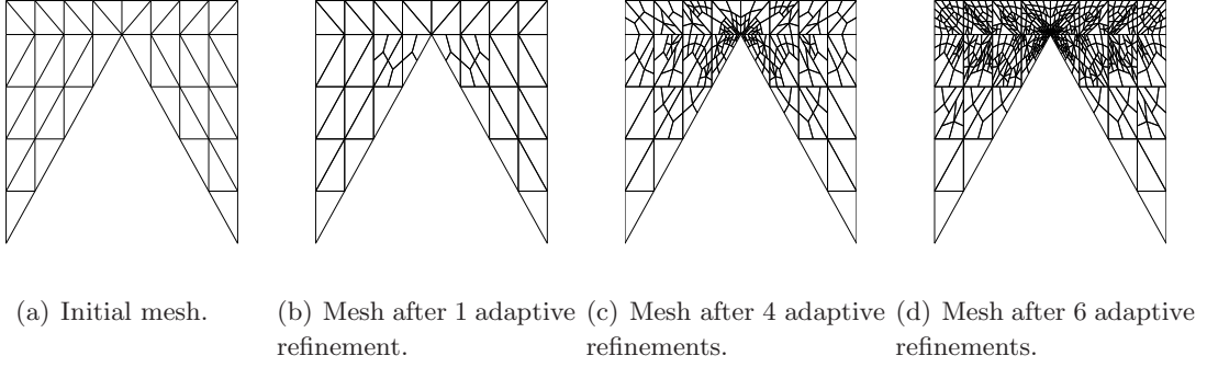
Figure 3.7: Test 2. Adaptively refined meshes for VEM scheme.
