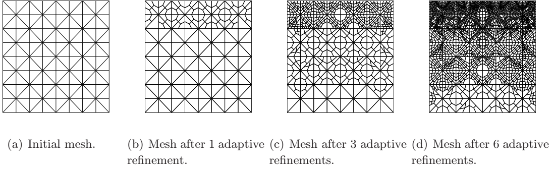
Figura 3.3: Test 1. Adaptively refined meshes for VEM scheme.
