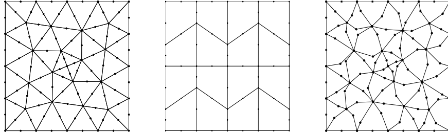
Figura 2.2: Test 1. Sample meshes: \mathcal{T}_h^1 (left), \mathcal{T}_h^2 (middle) and \mathcal{T}_h^3 (right) for N = 4 .
