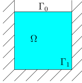
Figura 2.1: Sloshing in a square domain.
