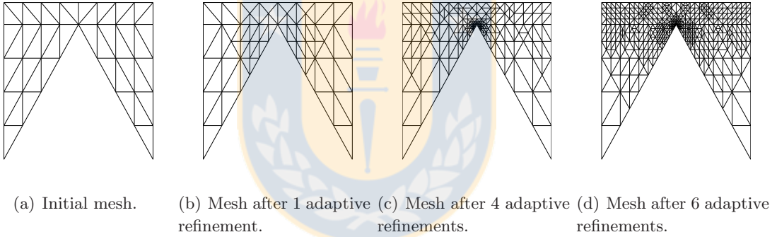
Figure 3.8: Test 2. Adaptively refined meshes for FEM scheme.
